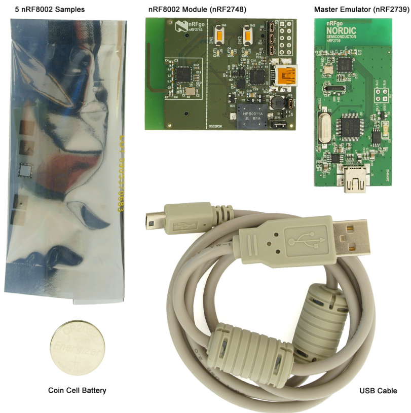
Figure 1. Hardware Content
